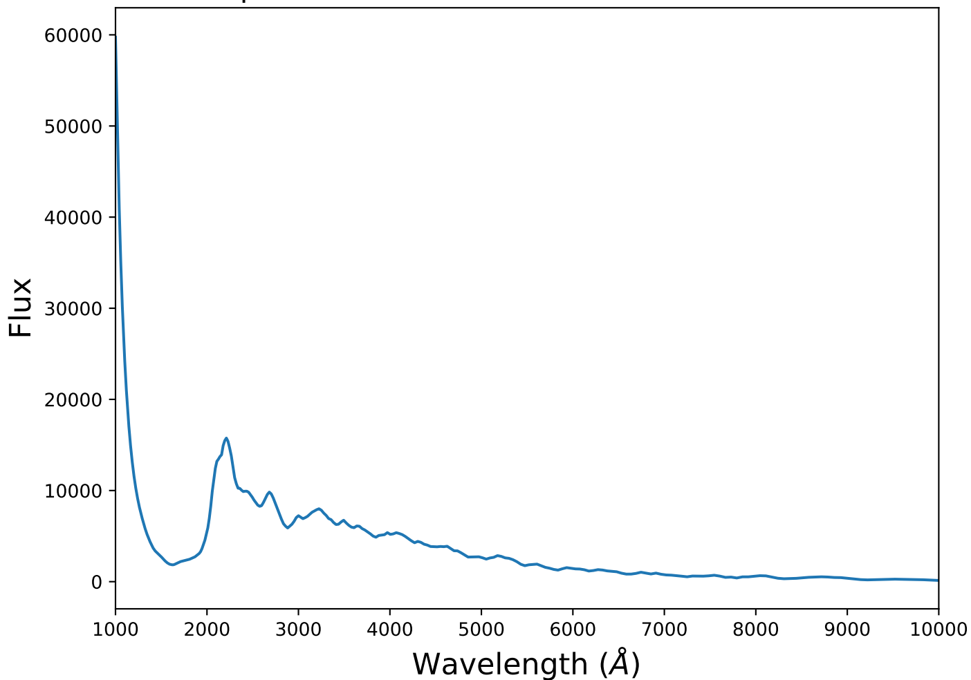
Spectrum 2 for transient SNIax at z=0.39
